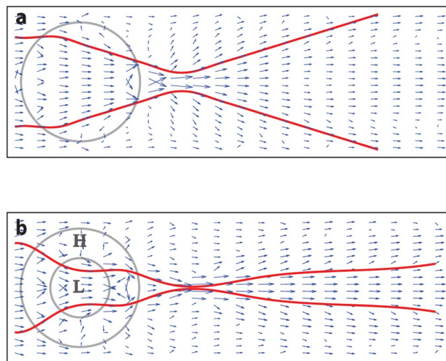
Fig. 1. Power flow plots for microspheres. (a) Single microsphere. (b) Two-layer microsphere. “L” and “H” denote the low index core and high index shell, respectively. The arrows denote the Poynting vector at each grid point. The two continuous red lines in each figure are the streamlines for the Poynting vector fields, assuming the same two fixed starting points on the incident side for each case.
