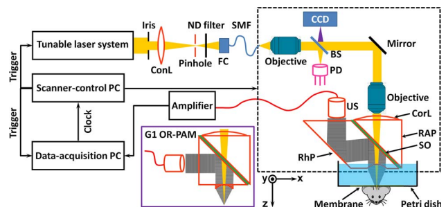
Fig. 1. (Color online) Schematic of G2 OR-PAM. The solid-boundary inset shows the configuration of the acoustic-optical combiner in G1 OR-PAM. ConL, condenser lens; ND, neutral density; FC, fiber collimator; SMF, single-mode fiber; CCD, charge-coupled device; BS, beam splitter; PD, photodiode; CorL, correction lens; RAP, right-angle prism; SO, silicone oil; RhP, rhomboid prism; US, ultrasonic transducer.
