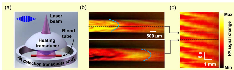
Fig. 2. Advance in PA deep tissue blood flow measurement. (a) Schematic of ultrasonically encoded photoacoustic flowgraphy, where part of the flowing blood is thermally tagged by a heating transducer. The movement of the tagged blood is imaged by a circular-array-based PA computed tomography system. (b) Snapshot PA images of the thermally tagged blood flowing in a plastic tube covered by 5-mm-thick chicken breast tissue. The two images are 9 seconds apart, and the flow is from left to right. The curved dashed line shows a parabolic heating peak propagating with blood flow. (c) Flow trajectories in the time-space plane, showing an en face spatial-temporal assembly of the measured temperature distribution of the flowing medium. Each horizontal line in the figure is extracted from one photoacoustic image along the flow direction, as shown by the black dashed line in (b). The flow speed and direction can be extracted from the slope of the trajectory. Adapted with permission from [22].
